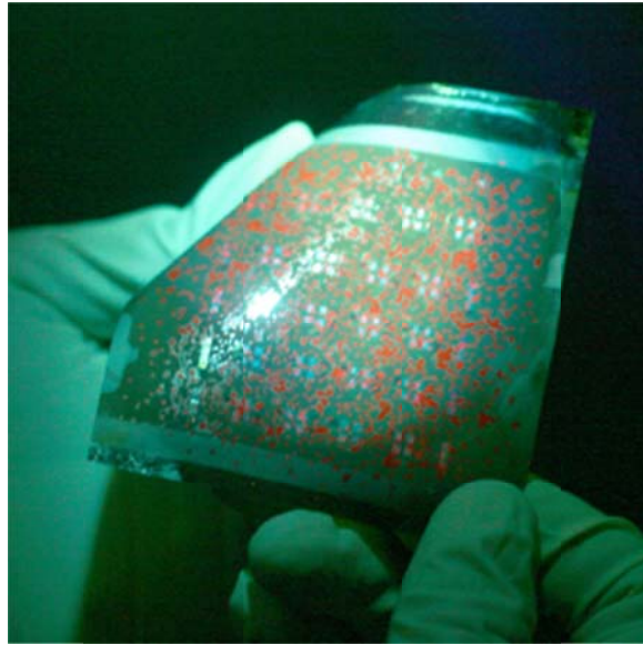
Figure 1: A highly thermostable organic transistor manufactured on a thin plastic film. The team succeeded in building a low drive-voltage and a highly thermostable organic circuit on a plastic film by using SAM molecule for the gate insulator, and high heat resistant semiconductors for semiconductor layer.
